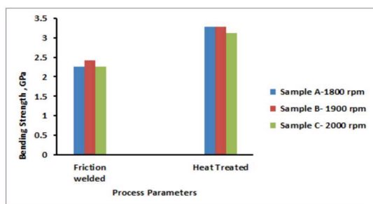
Fig 8: Bending strength of NiTiNol samples
